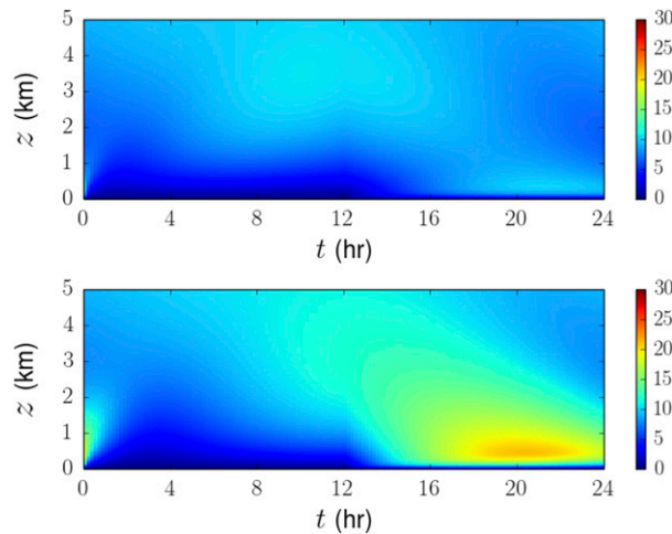
FIG. 2. Wind speed ( \text{m s}^{-1} ) as a function of time and height corresponding to the reference BH solutions for a 10 \text{ m s}^{-1} magnitude (top) northerly and (bottom) southerly free-atmosphere geostrophic wind. Times are hours after sunrise.
