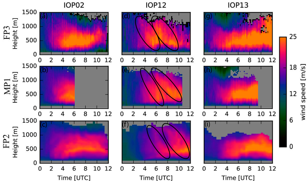
FIG. 5. Wind speed observations from (a),(d),(g) FP3, (b),(e),(h) MP1, and (c),(f),(i) FP2 are reproduced with diagonal striations during IOP12 highlighted by black circles. For reference, sunset occurred near 0200 UTC (2100 CDT) and sunrise occurred shortly after 1100 UTC (0600 CDT).
