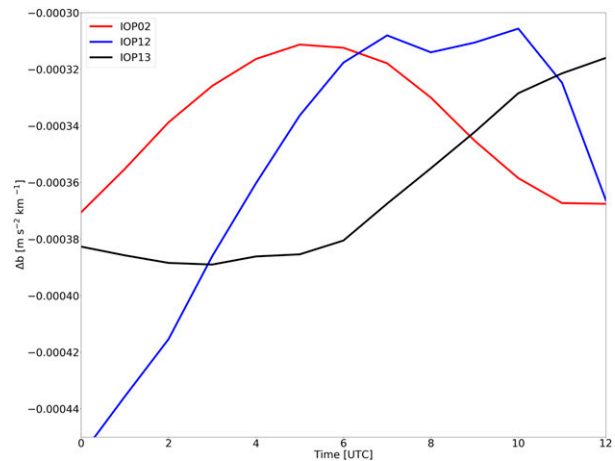
FIG. 18. Simulated buoyancy gradients between the west ( 36.5^\circ latitude, -100^\circ longitude) and east ( 36.5^\circ latitude, -95^\circ longitude) profile locations for PECAN IOPs 02, 12, and 13. For reference, sunset occurred near 0200 UTC (2100 CDT) and sunrise occurred shortly after 1100 UTC (0600 CDT).
