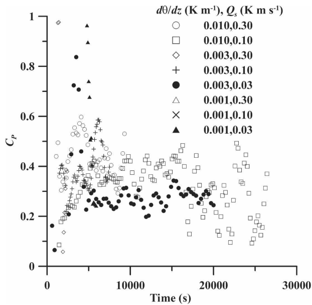
FIG. 16. The fraction of entrainment zone sheared-produced TKE used for entrainment in the GC case CBLs. The fraction was calculated by performing the integration illustrated in Fig. 5, which compared the integral change in the buoyancy flux profile expected from the NS case with the integral shear production in the entrainment zone and upper portion of the mixed layer. The output at all data points was averaged using the data point and five adjacent data points each on either side. For notation, see Fig. 14.
