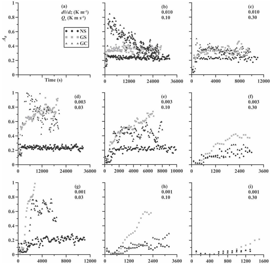
FIG. 8. Time series of the entrainment flux ratio A_R : (a) legend, (b)–(i) simulation results. The potential temperature lapse rate \partial\theta/\partial z ( \text{K m}^{-1} ) and the surface temperature flux Q_s ( \text{K m s}^{-1} ) are indicated in the upper right corner of each plot. Solid black circles show the NS case simulation data, gray squares the GS case data, and solid black triangles the GC case data.
