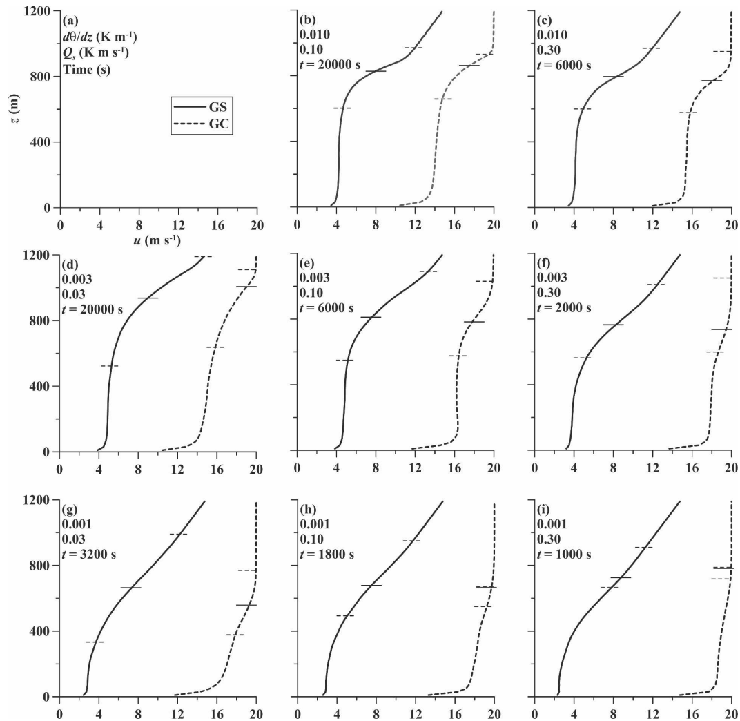
FIG. 6. Profiles of the x component of momentum at selected times during the simulation: (a) legend, (b)–(i) simulation results. The potential temperature lapse rate \partial\theta/\partial z ( \text{K m}^{-1} ), the surface temperature flux Q_s ( \text{K m s}^{-1} ), and the simulated elapsed time (s) are indicated in the upper left corner of each plot. The solid lines represent the profiles from the GS case simulations, and the dashed lines are from the GC case simulations. The CBL depth z_i is marked by a solid line on each profile, and the lower and upper limits of the entrainment zone are indicated by dashed lines.
