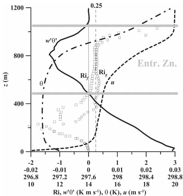
FIG. 12. Profiles of gradient Richardson number Ri_g (open circles), flux Richardson number Ri_f (open squares), potential temperature flux (solid black line), potential temperature (dot-dashed line), and the x component of momentum (dashed line) at t = 15\,000 s in the GC simulation with \partial\theta/\partial z = 0.003 K m ^{-1} and Q_s = 0.03 K m s ^{-1} .
