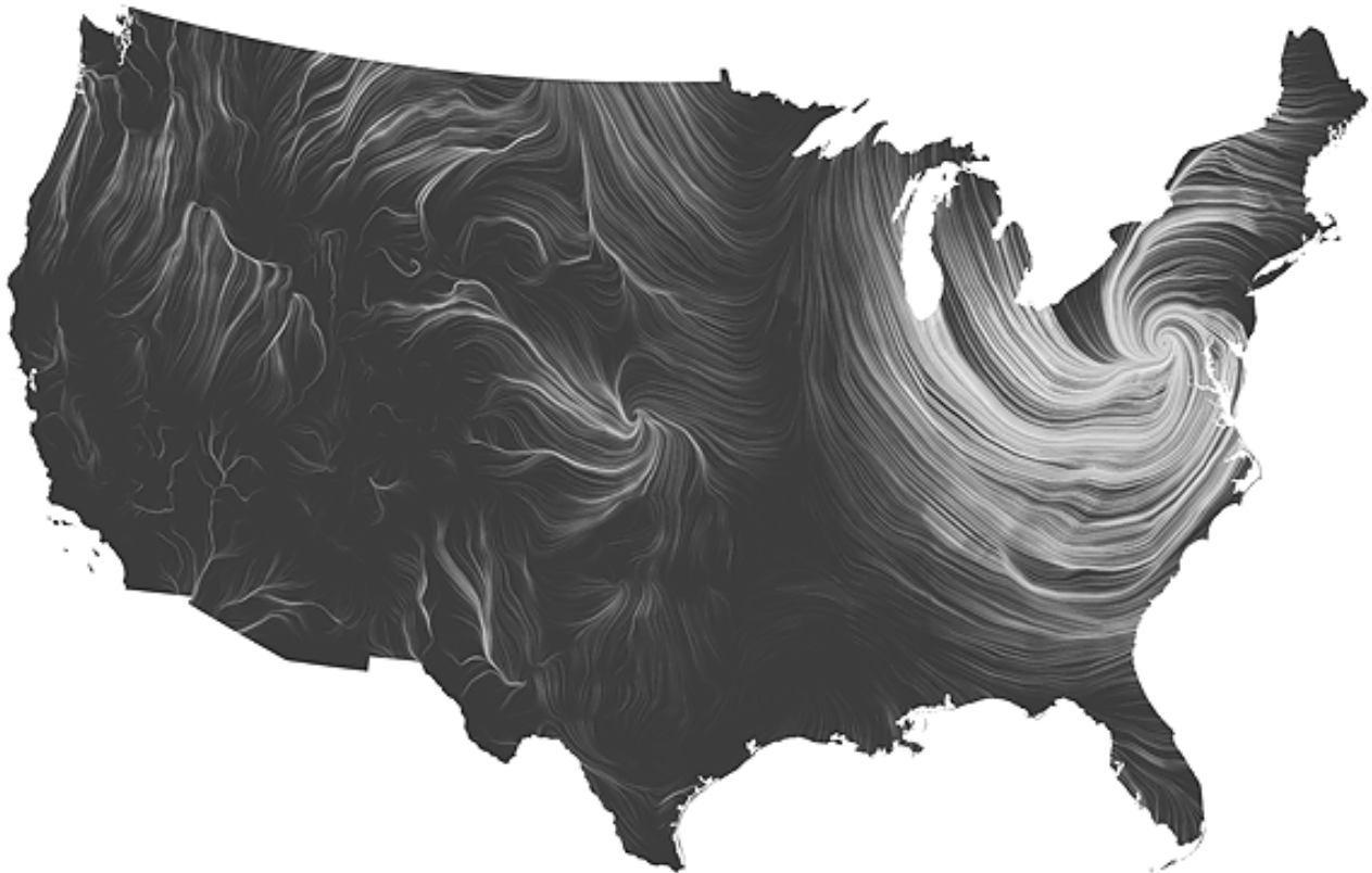
Streamline analysis (Hurricane Sandy after landfall, 30 Oct. 2012)
