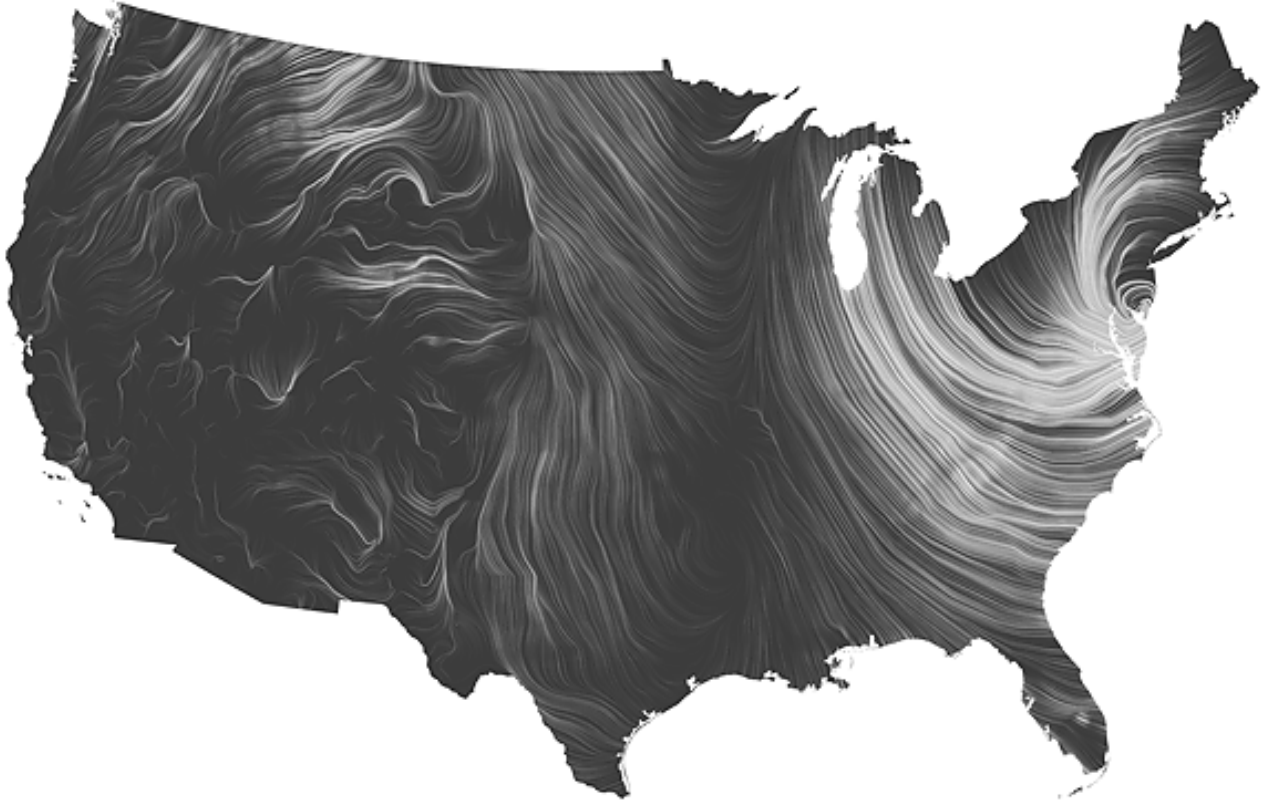
Streamline analysis (Hurricane Sandy before landfall, 29 Oct. 2012)
