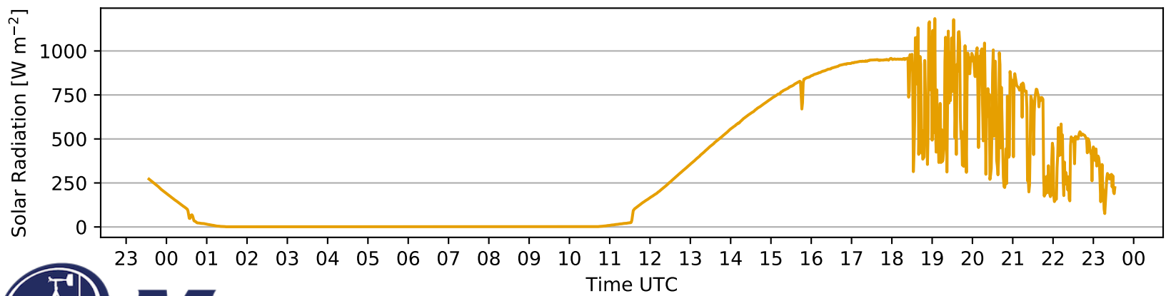
Solar Radiation
