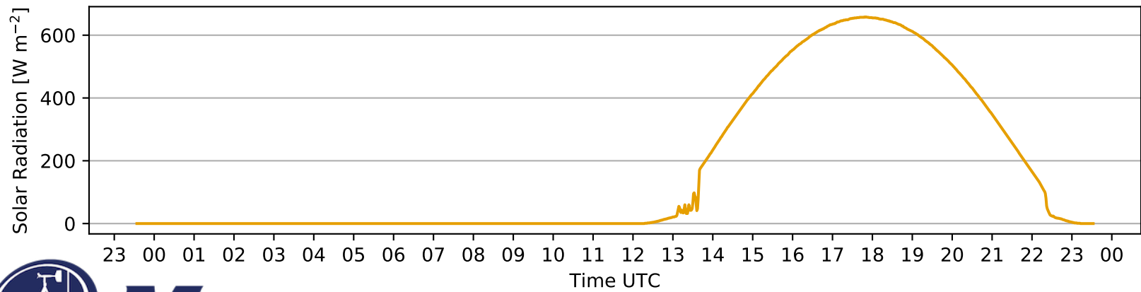
Solar Radiation
