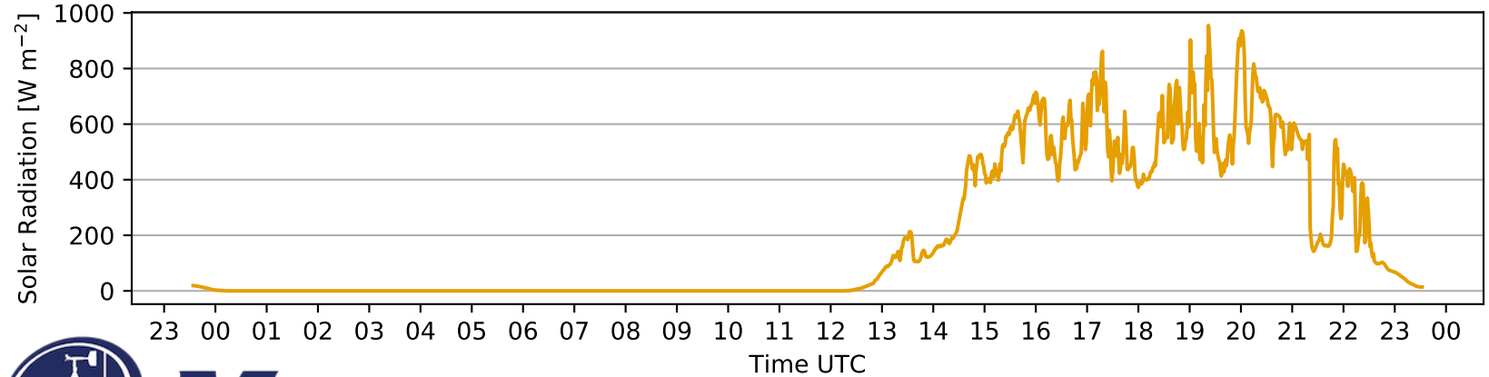
Solar Radiation
