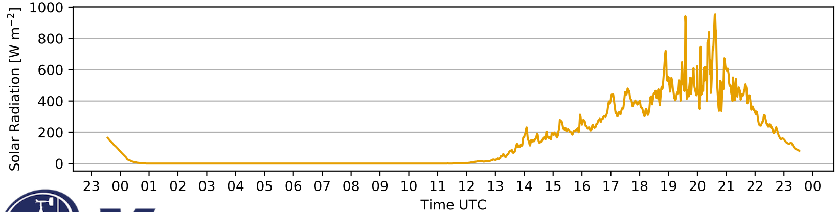
Solar Radiation
