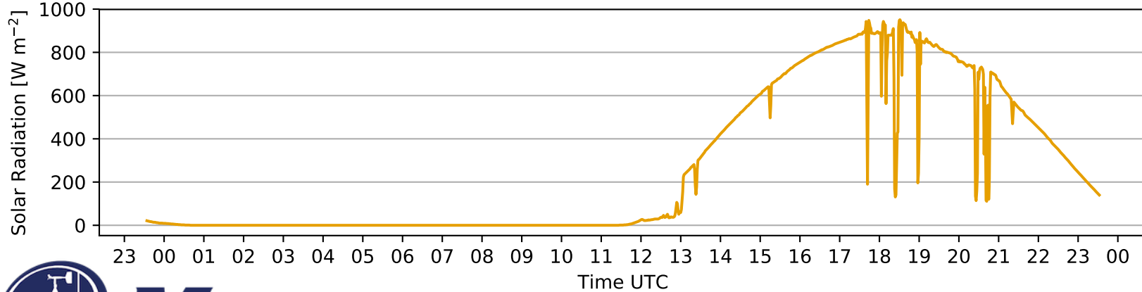
Solar Radiation
