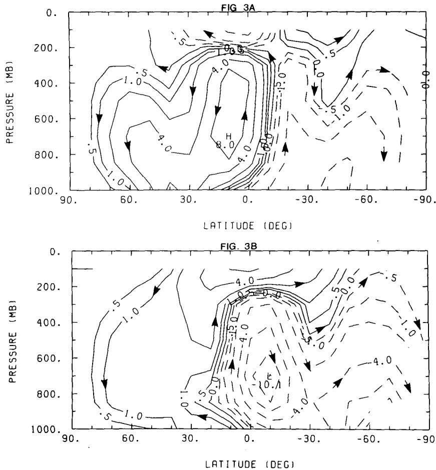
FIG. 3. Residual meridional streamfunction for (a) December-February and (b) June-August. Contours are drawn at values 0, \pm 0.5 , \pm 1.0 , \pm 2.0 , \pm 4.0 , \pm 6.0 , \dots \times 10^{17} \text{ m}^2 \text{ s Pa} and arrows indicate the direction of the circulation.
