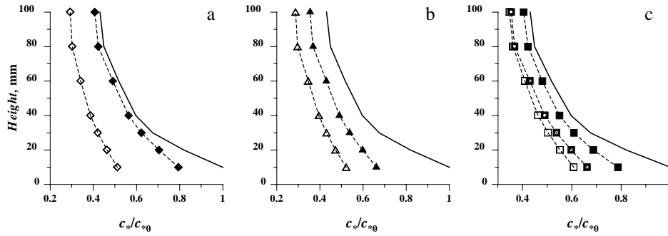
Figure 2. Wind tunnel data on the attenuation of concentration with (a) different wind velocities: u=4.9 m/s (open symbols) and u=10 m/s (filled symbols) with fixed v=12 m/s (43 km/h), and n_v=7 vehicles/100m; (b) different traffic velocities: v=17 m/s (61 km/h, open symbols) and v=12 m/s (43 km/h, filled symbols) with fixed u=7 m/s and n_v=7 vehicles/100m; (c) different traffic densities n_v=13 vehicles/100m (open symbols), n_v=7 vehicles/100m (half-filled symbols), and n_v=4 vehicles/100m (filled symbols) with fixed v/u=1.7 . Solid lines show the reference concentration profile without traffic, c_{s0} is the normalised concentration at the lowest position of corresponding reference profile.
