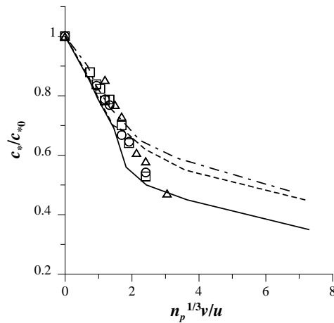
Figure 5. The wind tunnel data from Figure 4, points, compared with the numerical data of Stern and Yamartino (1998), lines. The numerical results refer to the situations with low traffic (solid line), medium traffic (dashed line), and high traffic (dashed and dotted line) according to classification by Stern and Yamartino (1998).
