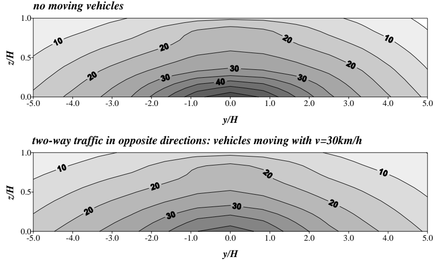
Figure 1. Values of c_* at the lee wall of the upwind building in the wind tunnel model of a street canyon without traffic (upper plot) and with two-way traffic in opposite directions (lower plot). For simulation details see section 3 and Kastner-Klein et al. (1998).
