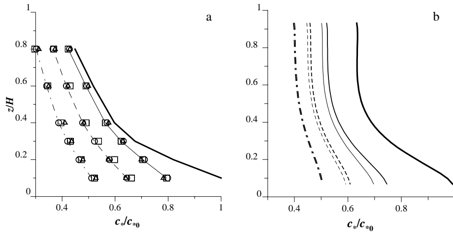
Figure 3. Concentration attenuation with different traffic-to-wind TKE production ratios as function of height normalized by the canyon depth H . In (a), are the wind tunnel data for P_t=1.7 (solid line), P_t=6.9 (dashed line), and P_t=13.8 (dashed and dotted line) with u from 4.9 to 14.2m/s, v from 6 to 24m/s, and n_v from 4 to 15 vehicles/100m. In (b) are numerical data for P_t=2.2 and 4.1 (solid lines), P_t=13.8 and 15.6 (dashed lines), and P_t=54.8 (dashed and dotted lines) with u=4\text{m/s} , v from 4 to 19m/s, and n_v from 4 to 19 vehicles/100m. Heavy solid lines show reference concentration profiles; c_{*0} is defined as in Figure 2.
