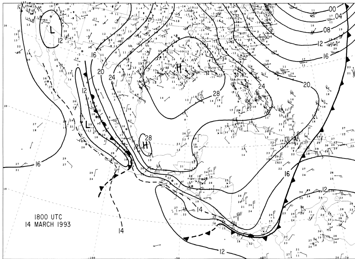
FIG. 16. Manually analyzed surface map for 1800 UTC 14 March. Notation as in Fig. 13.
