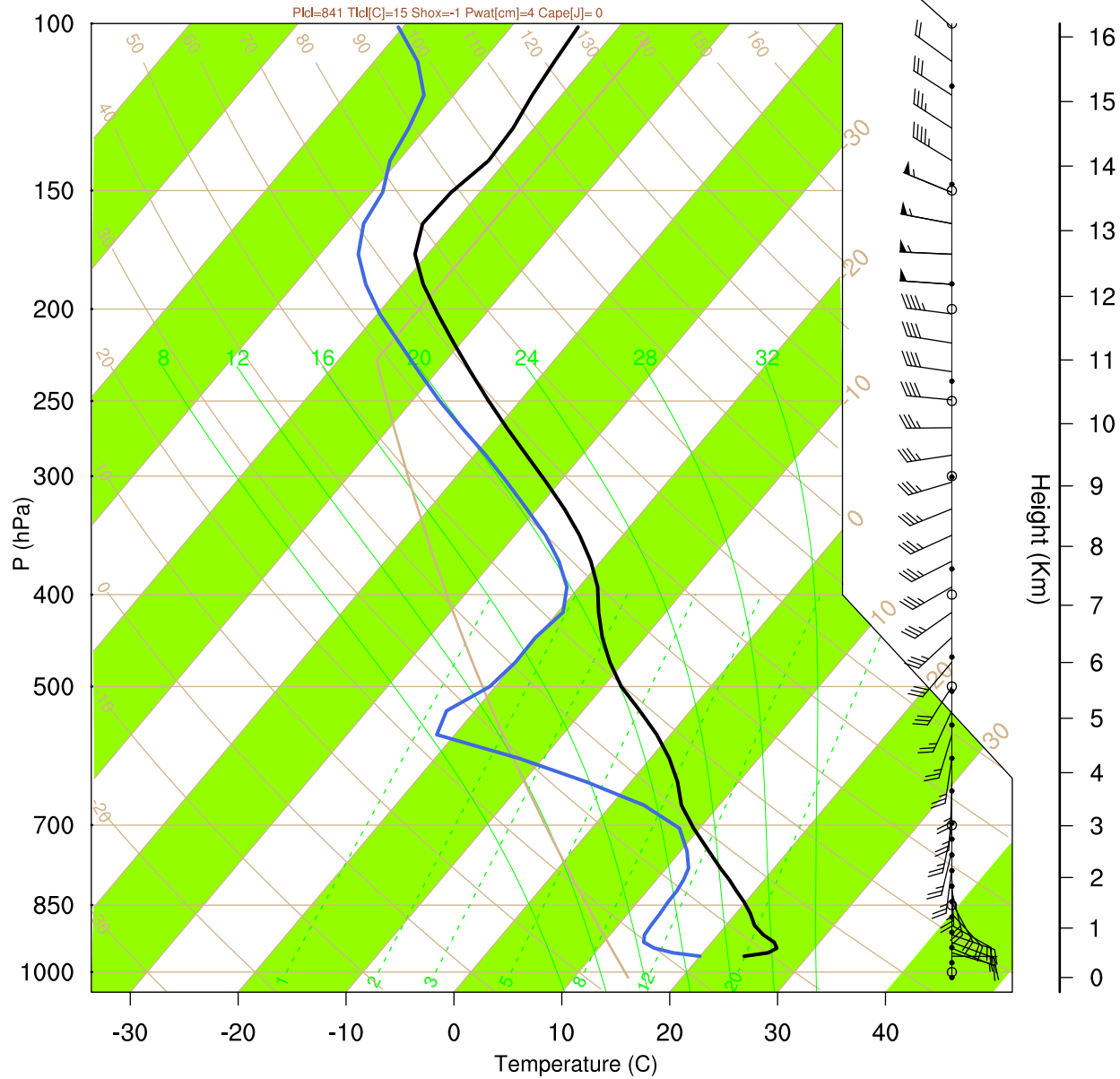
Plcl=841 Tlcl[C]=15 Shox=-1 Pwat[cm]=4 Cape[J]= 0
