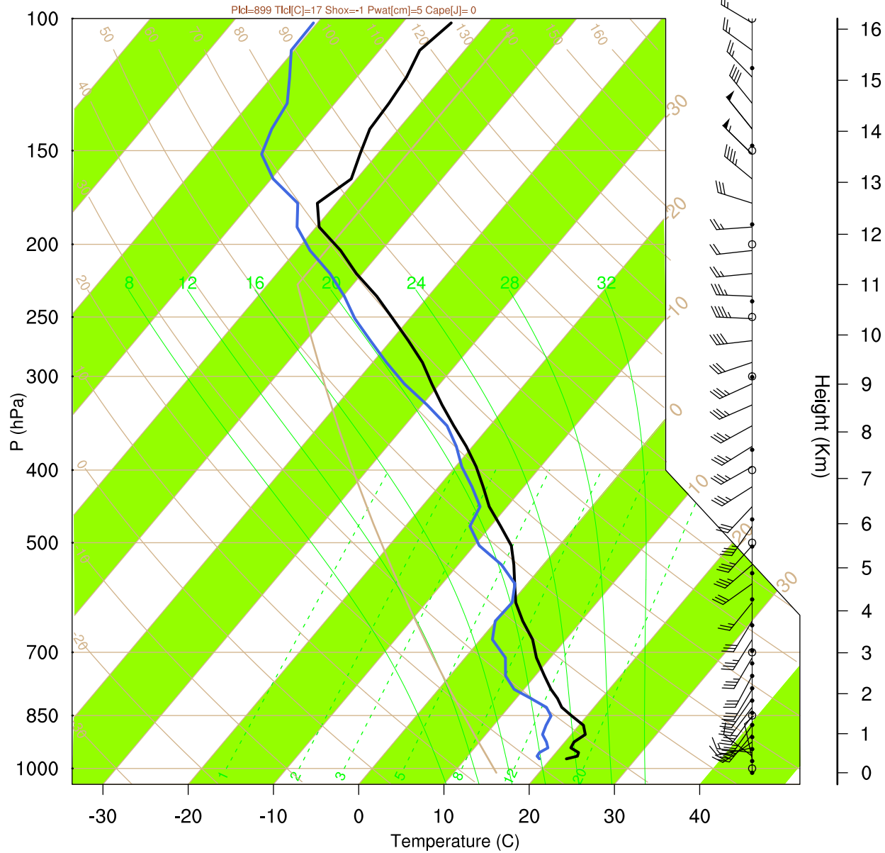
Plcl=899 Tlcl[C]=17 Shox=-1 Pwat[cm]=5 Cape[J]= 0
