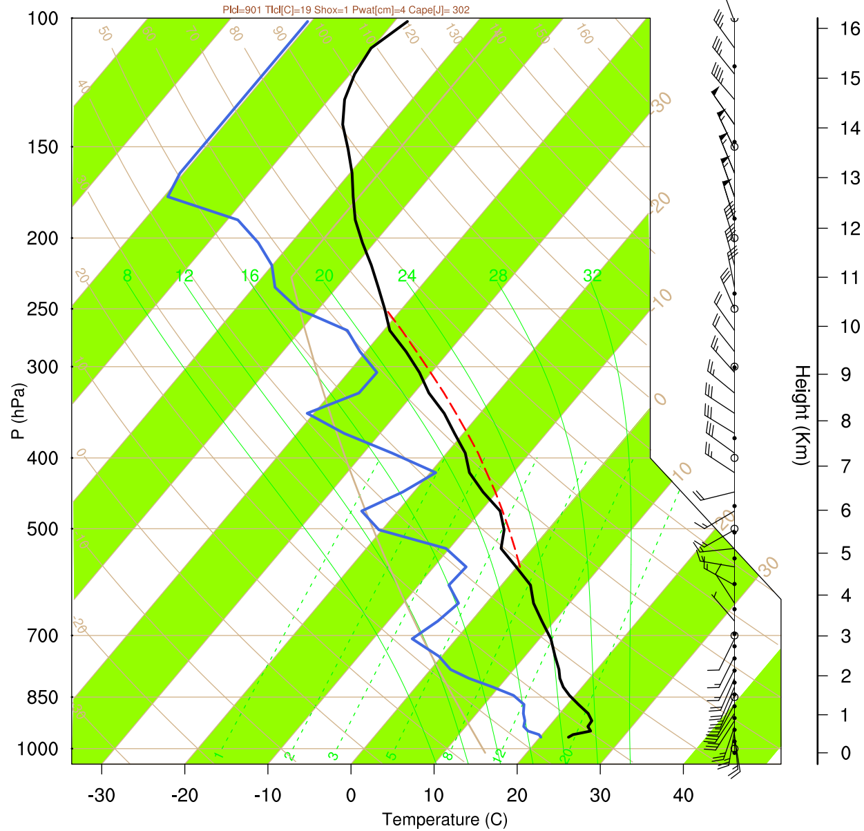
Norman (OK,USA) at 2015-06-11_12:00:00
