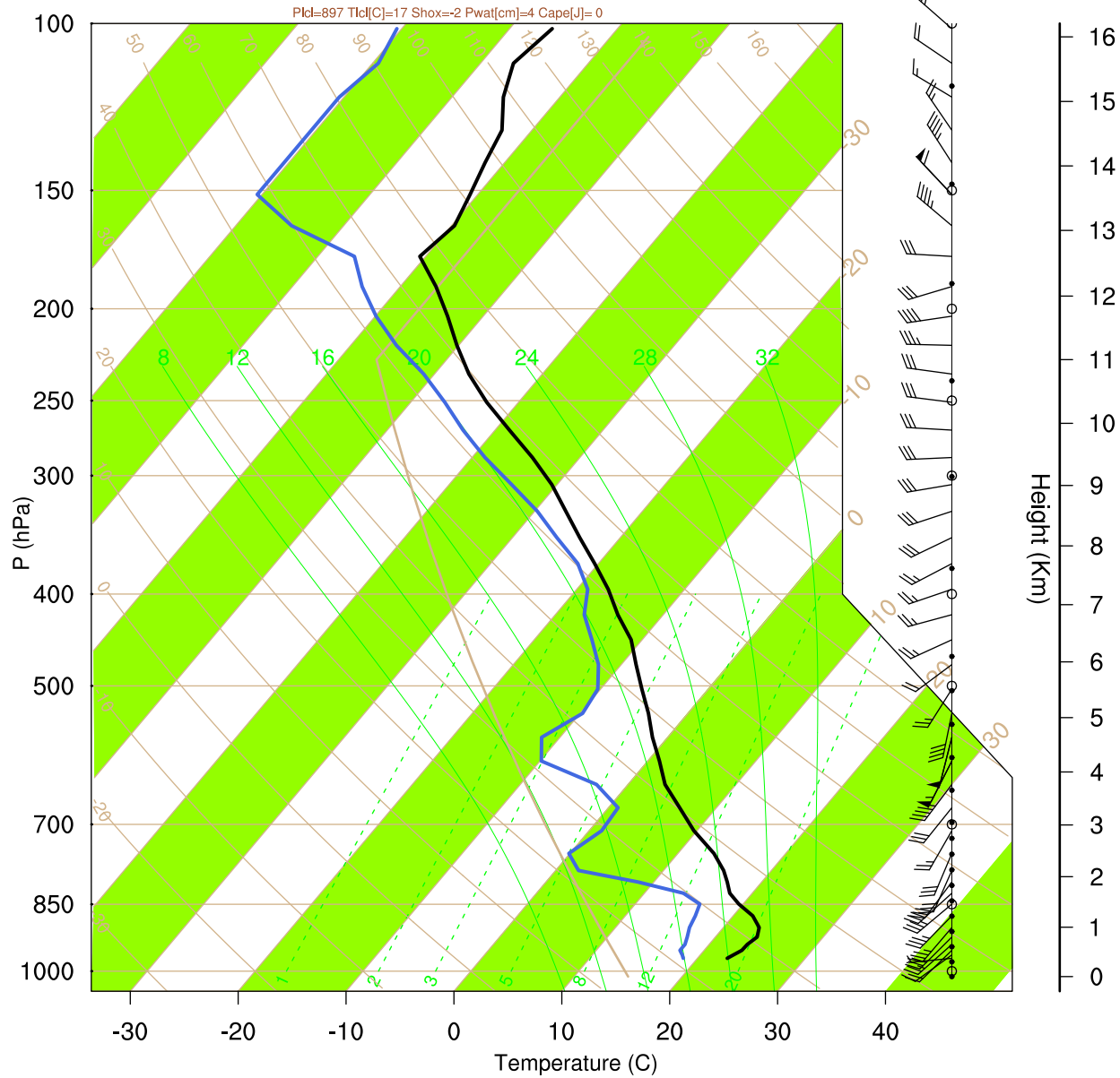
Plcl=897 Tlcl[C]=17 Shox=-2 Pwat[cm]=4 Cape[J]= 0
